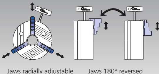
Jaws radially adjustable
